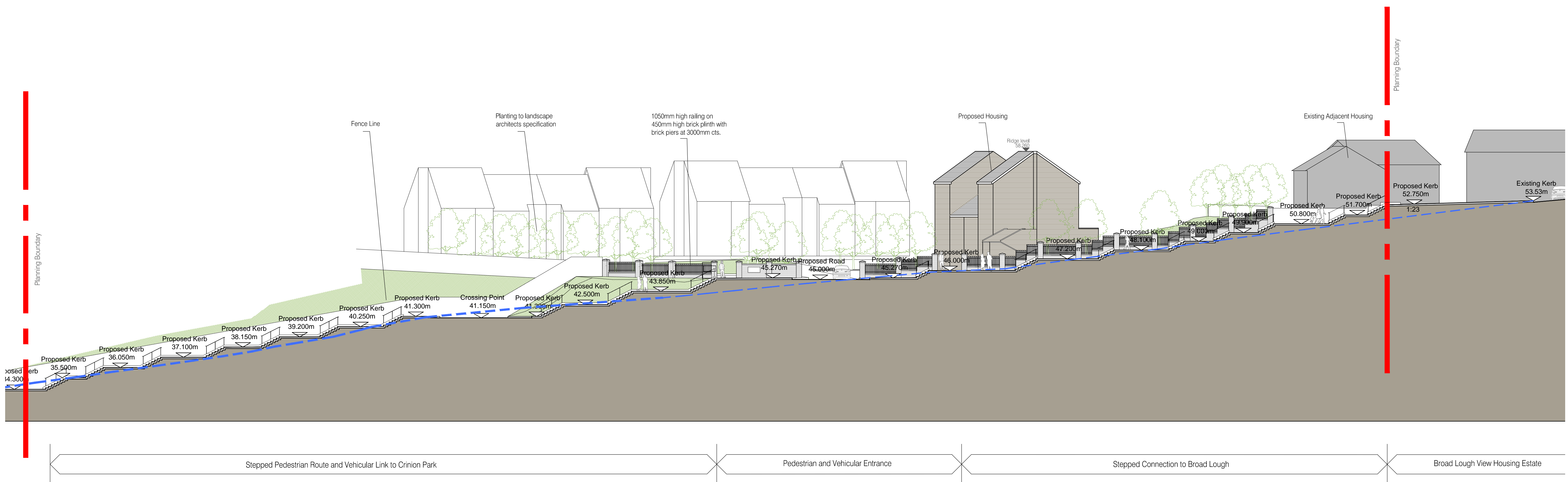
1 Northern Access Road Scale 1:200
